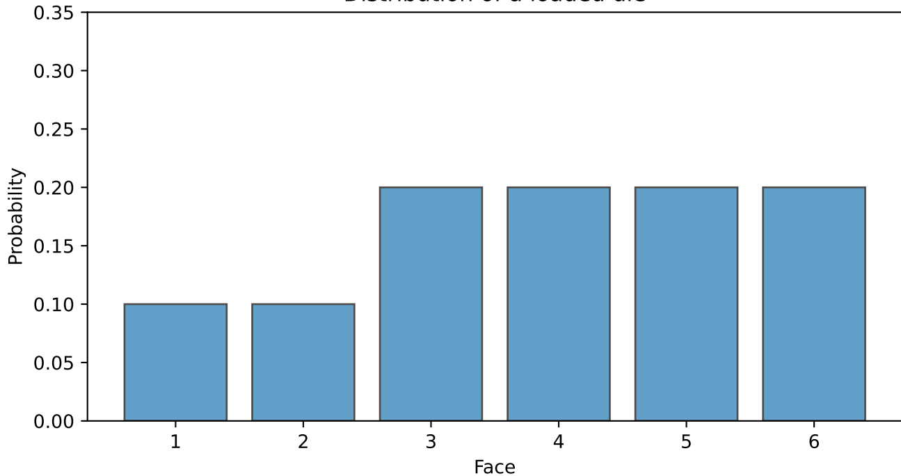
Distribution of a loaded die
